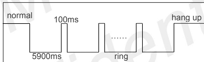
Figure 3: UART RI behavior when incoming call
